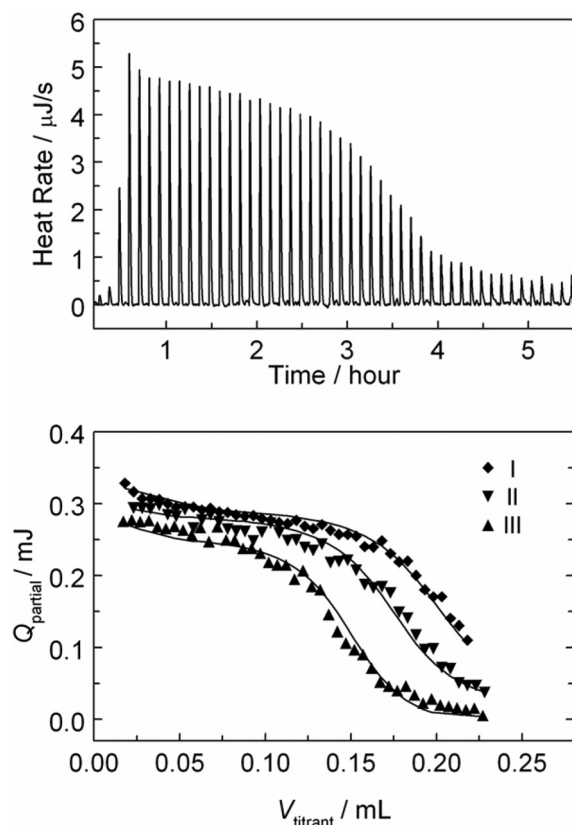
FIG. 5. Calorimetric titrations of the protonation of lactate, I = 1.05 \text{ mol} \cdot \text{kg}^{-1} \text{ NaClO}_4 , t = 25^\circ\text{C} . (Top) a representative thermogram. (Bottom) A plot of Q_{\text{partial}} vs. the volume of titrant, symbols – experimental Q , lines – fit; initial cup solutions: sodium lactate, C_{\text{NaL}}^0 ( \text{mmol} \cdot \text{dm}^{-3} ) = 22.22 (I), 19.44 (II), and 16.67 (III); titrant: 99.80 \text{ mmol} \cdot \text{dm}^{-3} \text{ HClO}_4 , 5.0 \mu\text{L}/\text{addition} .
