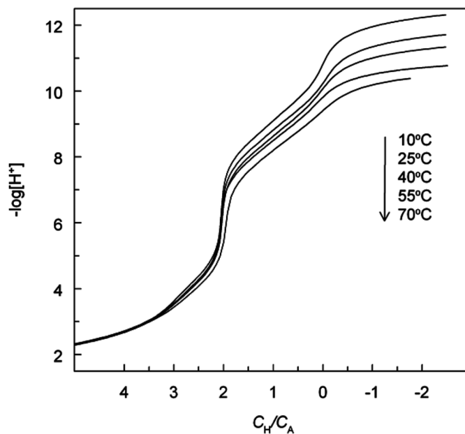
FIG. 1. Potentiometric titrations of DTPA protonation at different temperatures, I = 1.05 \text{ mol} \cdot \text{kg}^{-1} NaClO 4 . Cup solution: V^0 = 20.00 \text{ mL} , C_{\text{DTPA}}^0 = 6.665 \text{ mmol} \cdot \text{dm}^{-3} , C_H^0 = 33.34 \text{ mmol} \cdot \text{dm}^{-3} (for 10, 25, 40, and 55°C) and C_H^0 = 38.32 \text{ mmol} \cdot \text{dm}^{-3} (for 70°C). Titrant: 100.1 \text{ mmol} \cdot \text{dm}^{-3} NaOH. Negative values of C_H/C_A represent the region where hydroxide is in excess ( -C_H/C_A = C_{\text{OH}}/C_A ).
