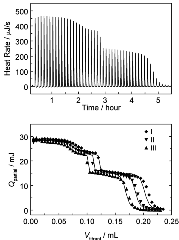
FIG. 6. Calorimetric titrations of the protonation of DTPA, I = 1.05 \text{ mol} \cdot \text{kg}^{-1} \text{ NaClO}_4 , t = 25^\circ\text{C} . (Top) a representative thermogram. (Bottom) A plot of Q_{\text{partial}} vs. the volume of titrant, symbols – experimental Q , lines – fit; initial cup solutions: DTPA, C_{\text{H}}^0/C_{\text{A}}^0 ( \text{mmol} \cdot \text{dm}^{-3} ) = 22.22/4.440 (I), 20.38/4.076 (II) and 18.50/3.700 (III); titrant: 100.0 \text{ mmol} \cdot \text{dm}^{-3} \text{ NaOH} , 5.0 \mu\text{L}/\text{addition} .
