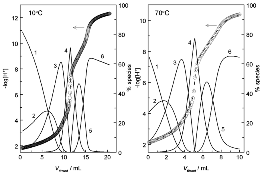
FIG. 3. Representative potentiometric titrations of the protonation of DTPA at 10°C (left) and 70°C (right), I = 1.05 \text{ mol} \cdot \text{kg}^{-1} \text{ NaClO}_4 . Cup solution: for 10°C, V^\circ = 30.00 \text{ mL} , C_{\text{DTPA}}^\circ = 6.667 \text{ mmol} \cdot \text{dm}^{-3} ; C_{\text{H}}^\circ = 50.00 \text{ mmol} \cdot \text{dm}^{-3} ; for 70°C, V^\circ = 20.00 \text{ mL} , C_{\text{DTPA}}^\circ = 6.665 \text{ mmol} \cdot \text{dm}^{-3} ; C_{\text{H}}^\circ = 38.32 \text{ mmol} \cdot \text{dm}^{-3} . Titrant: 100.1 \text{ mmol} \cdot \text{dm}^{-3} \text{ NaOH} . Symbols: (○ – experimental data ( -\log[\text{H}^+] ), dashed line – fit ( -\log[\text{H}^+] ); solid lines – percentage of DTPA species (right y-axis), \text{H}_5\text{A} (1), \text{H}_4\text{A}^- (2), \text{H}_3\text{A}^{2-} (3), \text{H}_2\text{A}^{3-} (4), \text{HA}^{4-} (5), and \text{A}^{5-} (6), where \text{H}_5\text{A} stands for the neutral DTPA acid.
