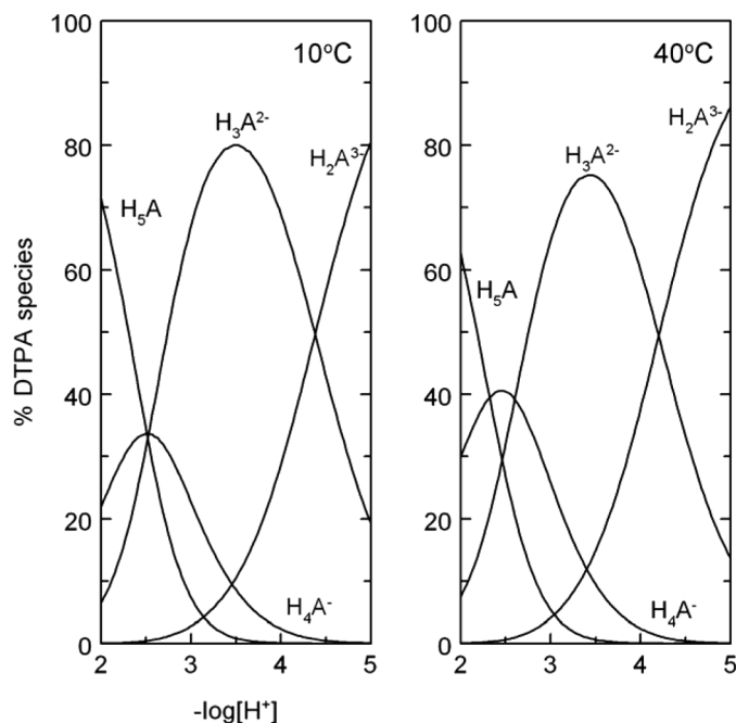
FIG. 7. Speciation of DTPA as a function of acidity ( -\log[H^+] ) at different temperatures. I = 1.05 \text{ mol} \cdot \text{kg}^{-1} \text{ NaClO}_4 , C_{\text{DTPA}} = 0.05 \text{ mol} \cdot \text{dm}^{-3} . Lines: percentage of DTPA species ( \text{H}_5\text{A} , \text{H}_4\text{A}^- , \text{H}_3\text{A}^{2-} , and \text{H}_2\text{A}^{3-} ). The \text{H}_4\text{A}^- and \text{A}^{5-} species are insignificant in the region of -\log[H^+] = 2 - 5 .
