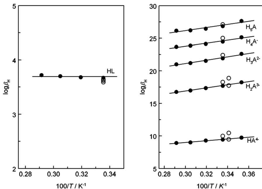
FIG. 4. Protonation constants of lactate (left) and DTPA (right) at different temperatures, I = 1.05 \text{ mol} \cdot \text{kg}^{-1} \text{ NaClO}_4 . Solid symbols: data from this work; open symbols, data from the literature [10]; lines: linear fits of the data from this work.
