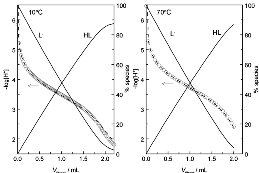
FIG. 2. Representative potentiometric titrations of the protonation of lactate at 10°C (left) and 70°C (right), I = 1.05 \text{ mol} \cdot \text{kg}^{-1} \text{ NaClO}_4 . Cup solution: V^\circ = 20.00 \text{ mL} , 0.100 \text{ mol} \cdot \text{dm}^{-3} sodium lactate. Titrant: 0.9994 \text{ HClO}_4 . Symbols: (○ – experimental data ( -\log[\text{H}^+] ), dashed line – fit ( -\log[\text{H}^+] ); solid lines – percentage of lactate species ( \text{L}^- and HL, where HL stands for the neutral lactic acid).
